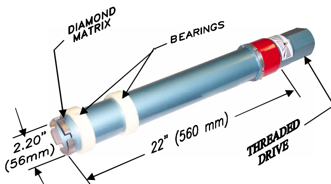
DB1 DRILL BIT
